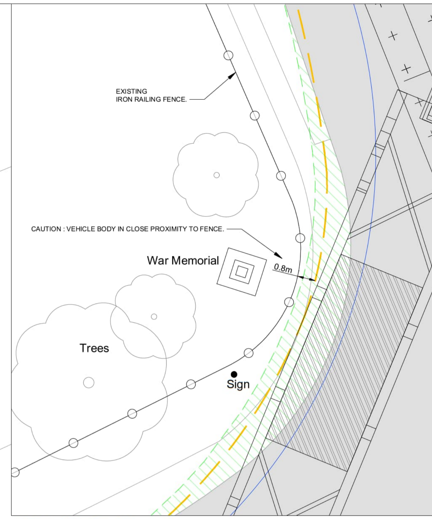
DETAIL (SCALE 1:100)
