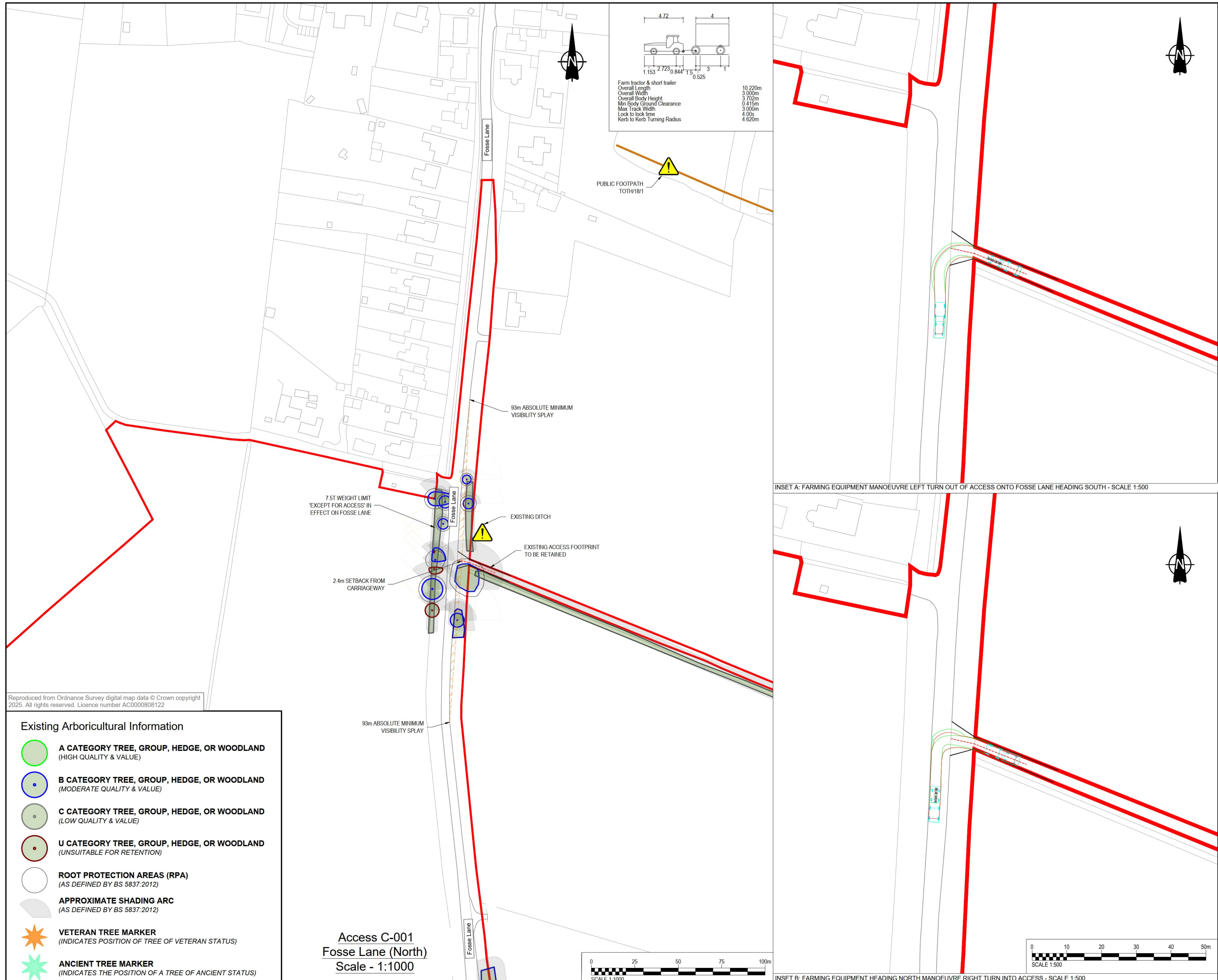
INSET B: FARMING EQUIPMENT HEADING NORTH MANOEUVRE RIGHT TURN INTO ACCESS - SCALE 1:500
