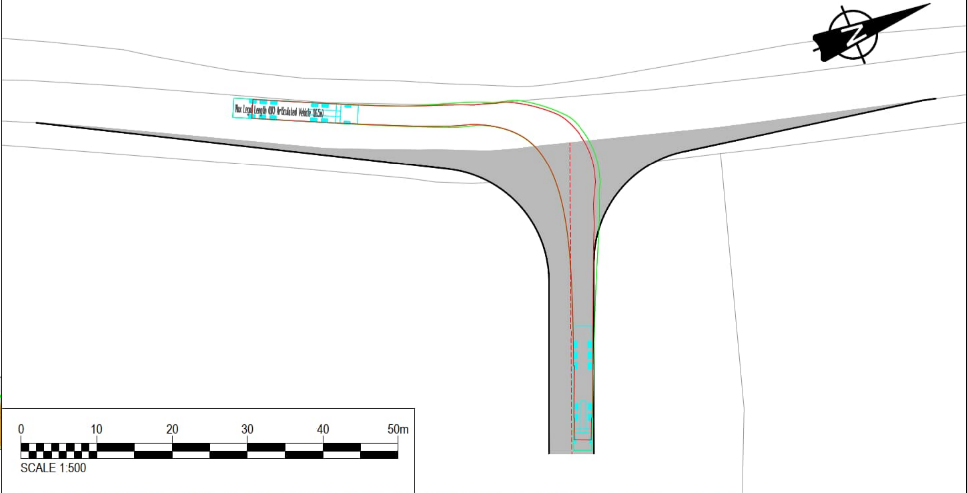
INSET D: ARTICULATED VEHICLE HEADING NORTH ON HADDINGTON LANE RIGHT TURN INTO ACCESS - SCALE 1:500
