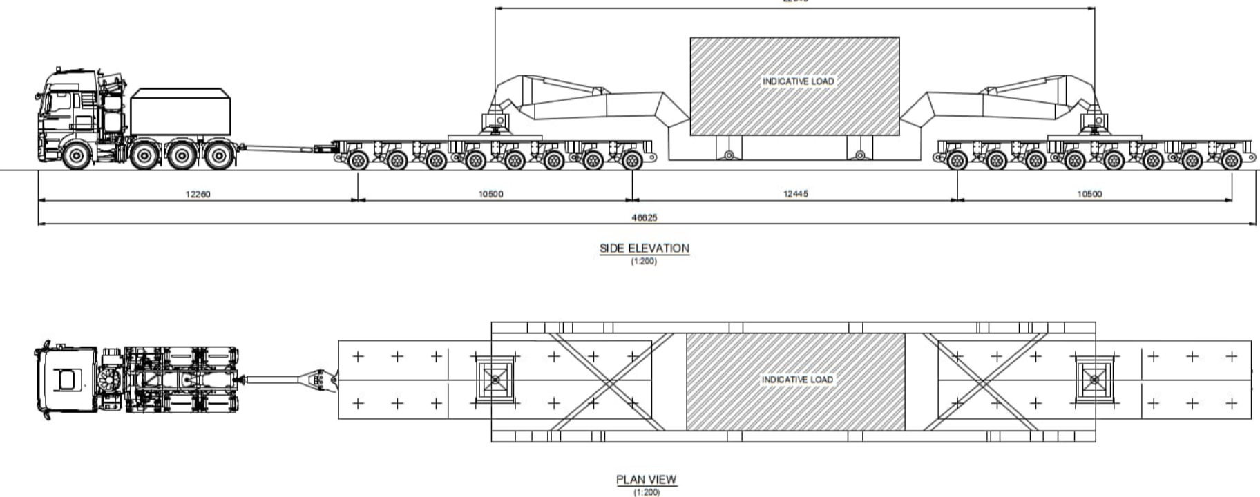
VEHICLE CONFIGURATION - 16-AXLE GIRDER TRAILER (Refer notes)
