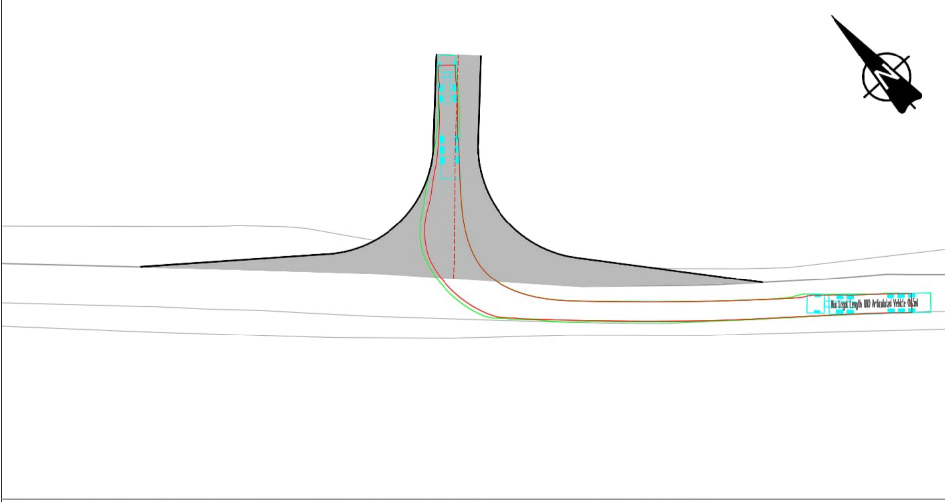
INSET C: ARTICULATED VEHICLE HEADING WEST ON BASSINGHAM ROAD RIGHT TURN INTO ACCESS - SCALE 1:500
