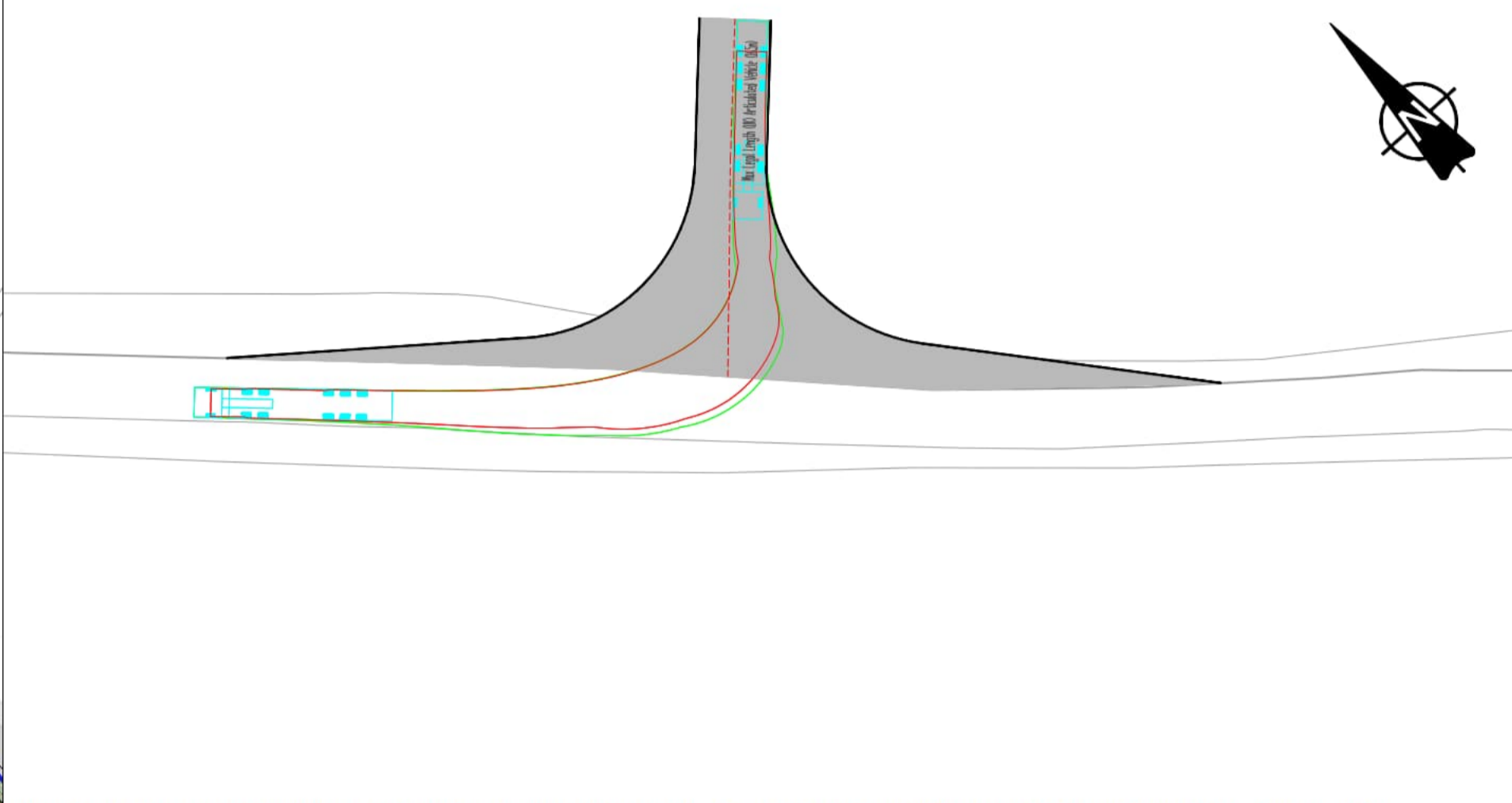
INSET B: ARTICULATED VEHICLE MANOEUVRE RIGHT TURN OUT OF ACCESS ONTO BASSINGHAM ROAD HEADING WEST - SCALE 1:500
