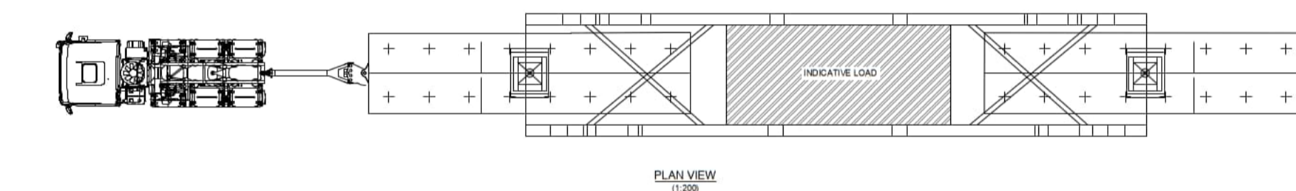
VEHICLE CONFIGURATION - 16-AXLE GIRDER TRAILER (Refer notes)
