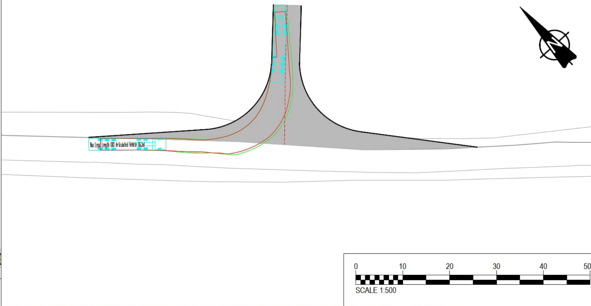
INSET D: ARTICULATED VEHICLE HEADING EAST ON BASSINGHAM ROAD LEFT TURN INTO ACCESS - SCALE 1:500
